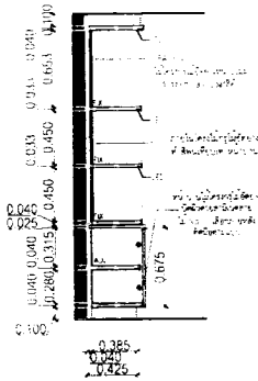
SECTION S-1 SCALE 1:50
