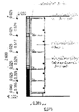
SECTION S-3 SCALE 1:50
