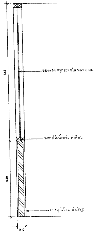
9 SECTION 10-11 SCALE 1:15
