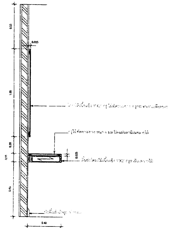
6 SECTION 10-09
