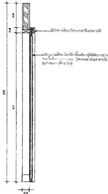
5 SECTION 10-09
