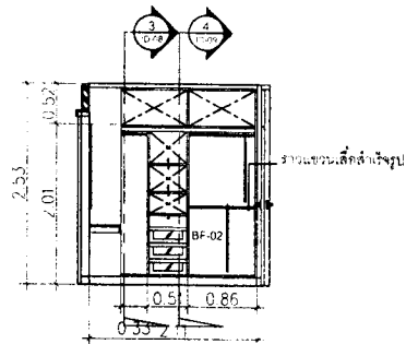
E ELEVATION 1:50 ID-06 INSIDE CLOSET
