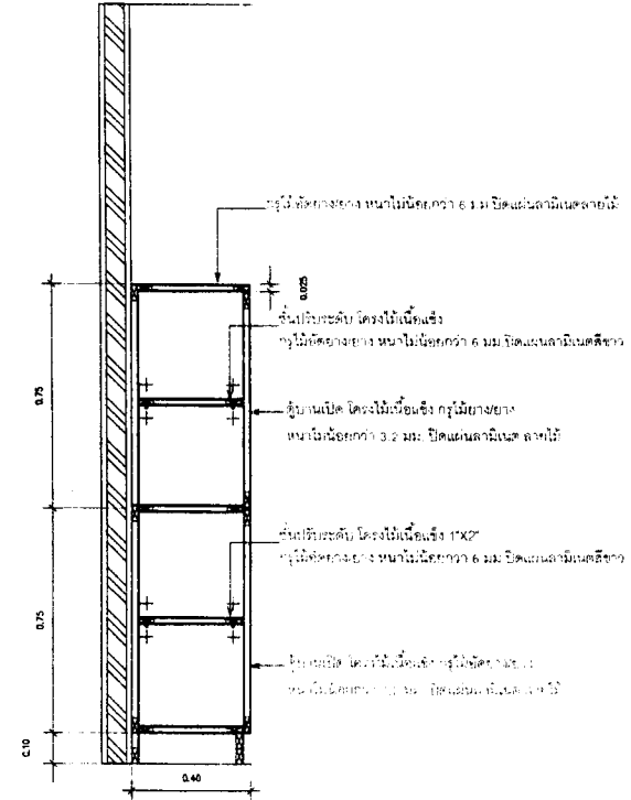
8 SECTION D-10 SCALE
