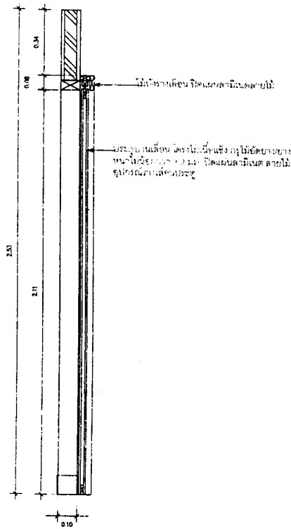
5 SECTION 10-09 SCALE 1:10
