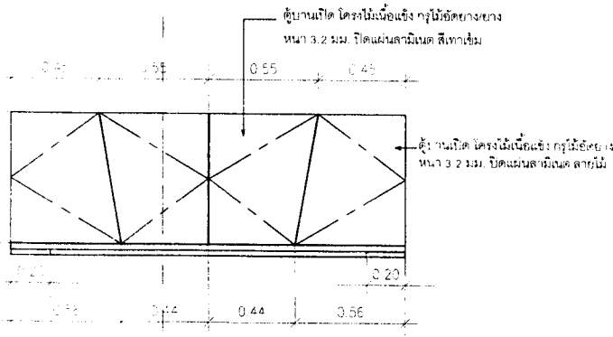
FRONT VIEW SCALE 1:25
