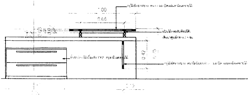
1 ID-14 DETAIL SCALE
