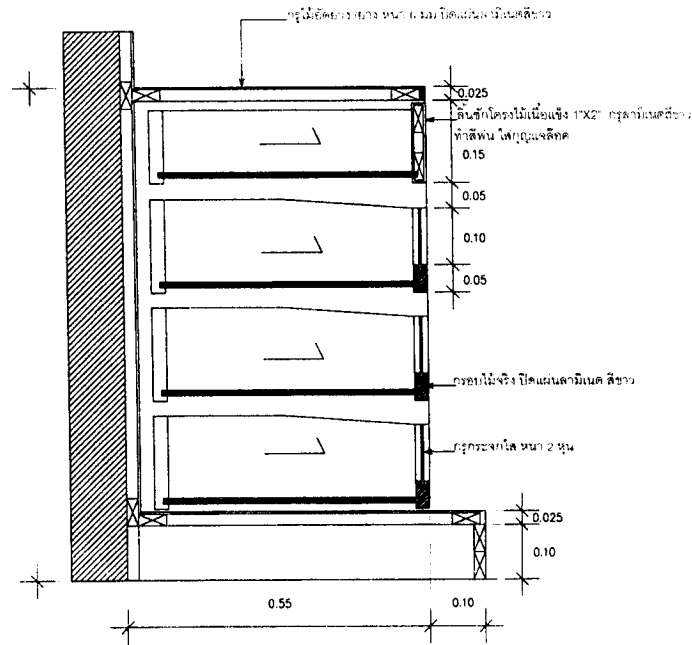
10 DETAIL 10-11 SCALE 1:10
