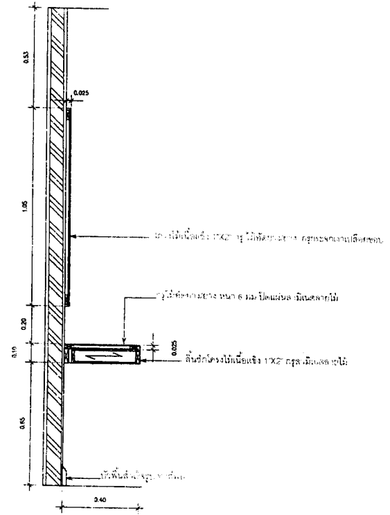
6 SECTION 10-09 SCALE 1:10
