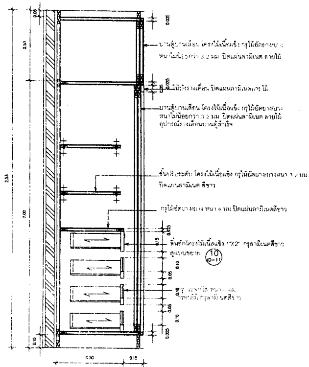
4 SECTION 10-09
