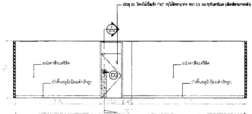
L 10-07 ELEVATION 1: 50
