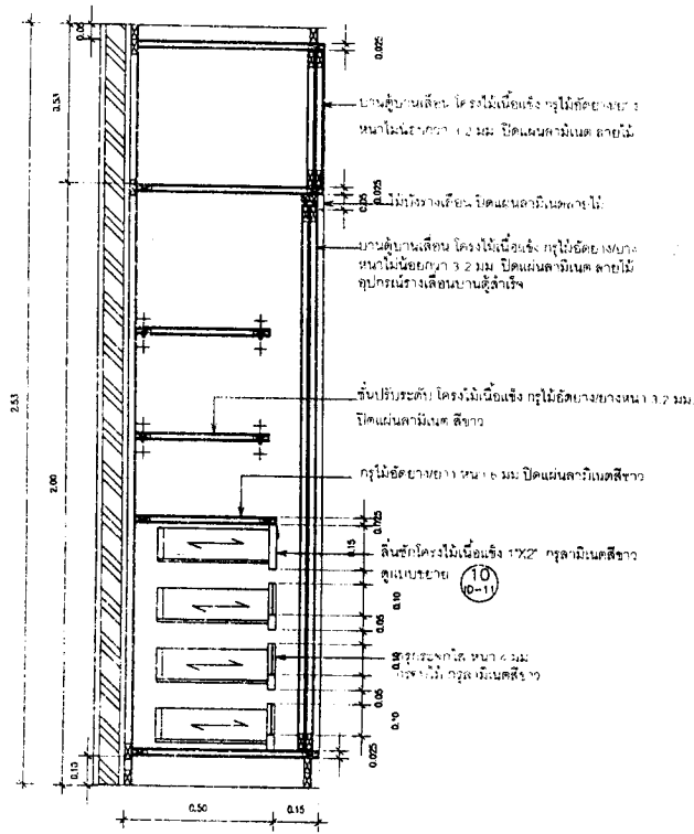
4 SECTION 10-09 SCALE 1:10
