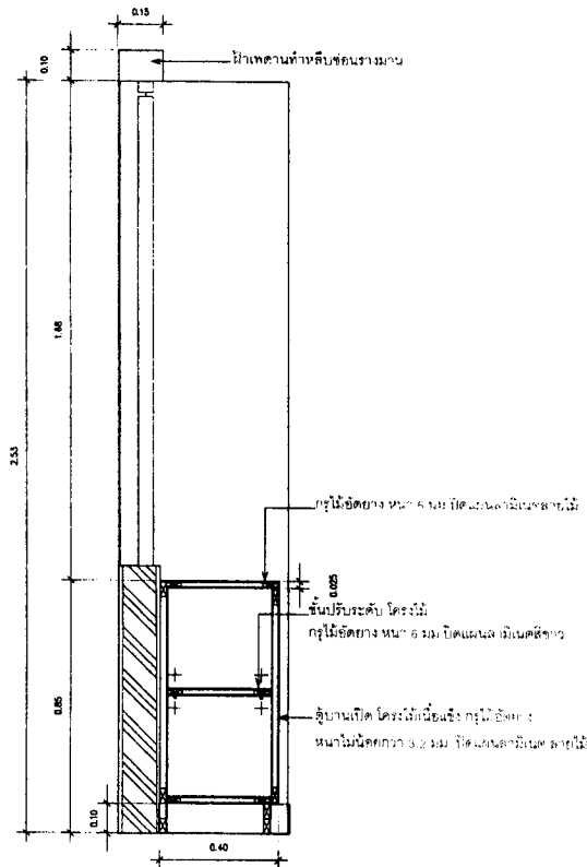
2 SECTION D-06 SCALE 1:15
